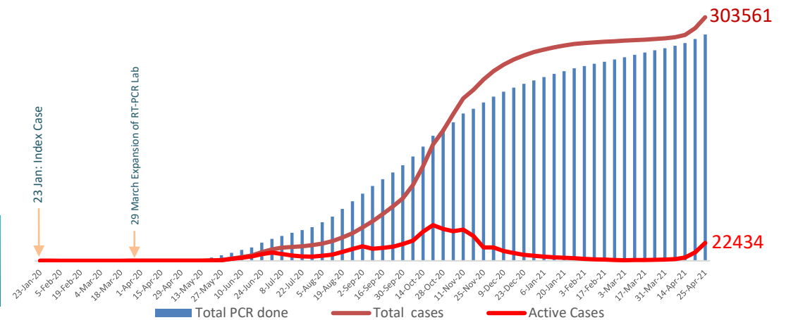
Trend of RT-PCR and COVID-19 cases
